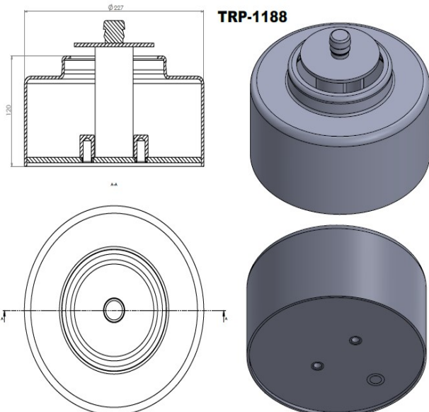
TRP-1188 BMC NEOCITY FRONT AIR SPRING LOWER PISTON
