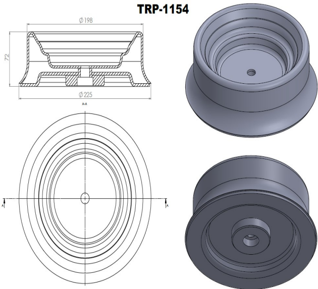
TRP-1154 AIR SPRING PISTON
